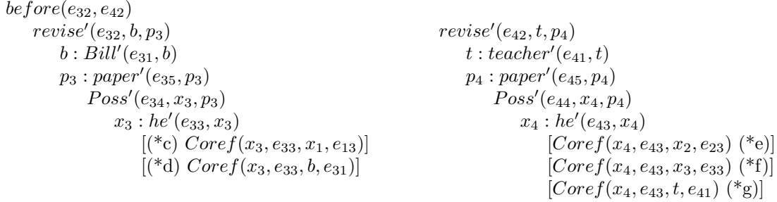
Figure 3: Representations for Five Readings Case
